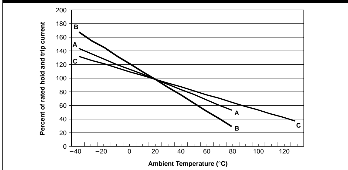
Figure S1. Thermal Derating Curve
